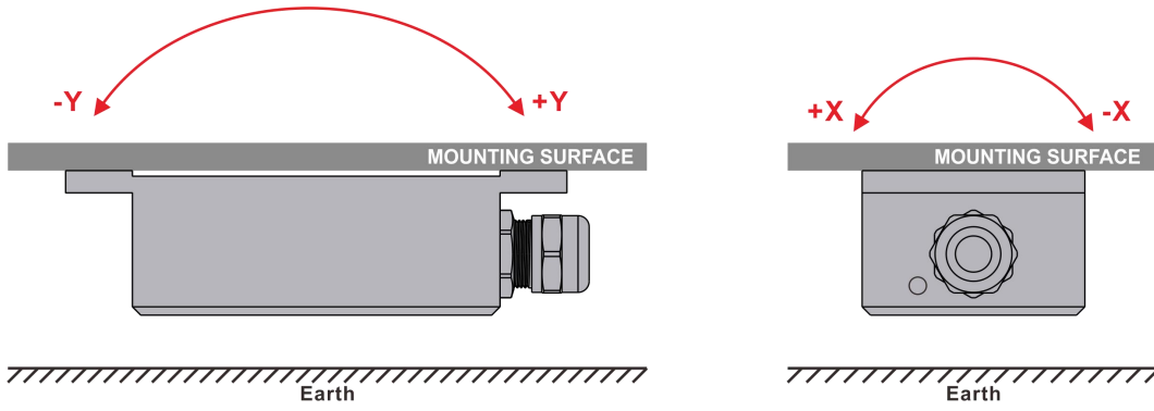
Horizontal-down installation
