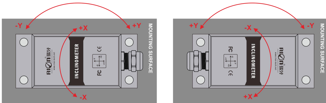
Vertical-left installation
